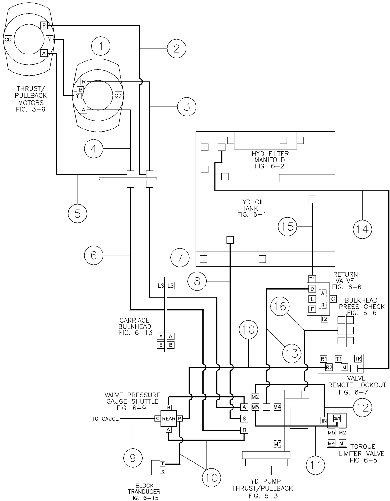
Thrust/Pullback Fig 12-2
