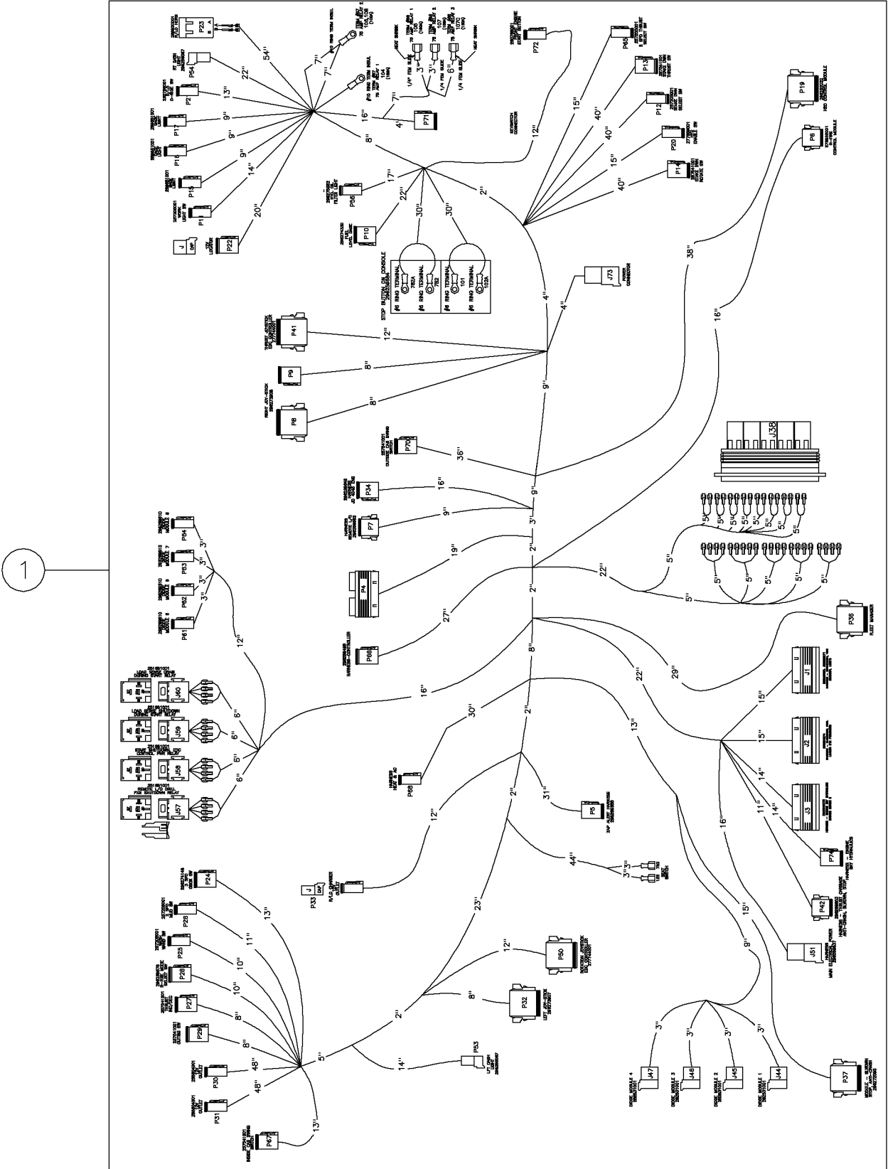
Harness-Console Fig 4-22
