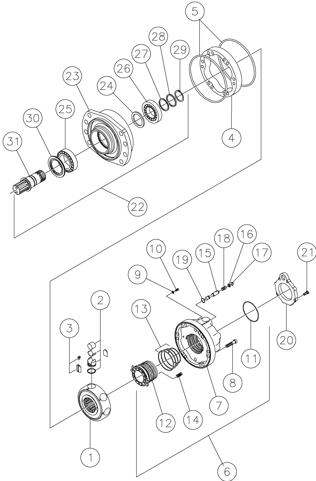
Components-Rotation Motor Fig 3-12z01
