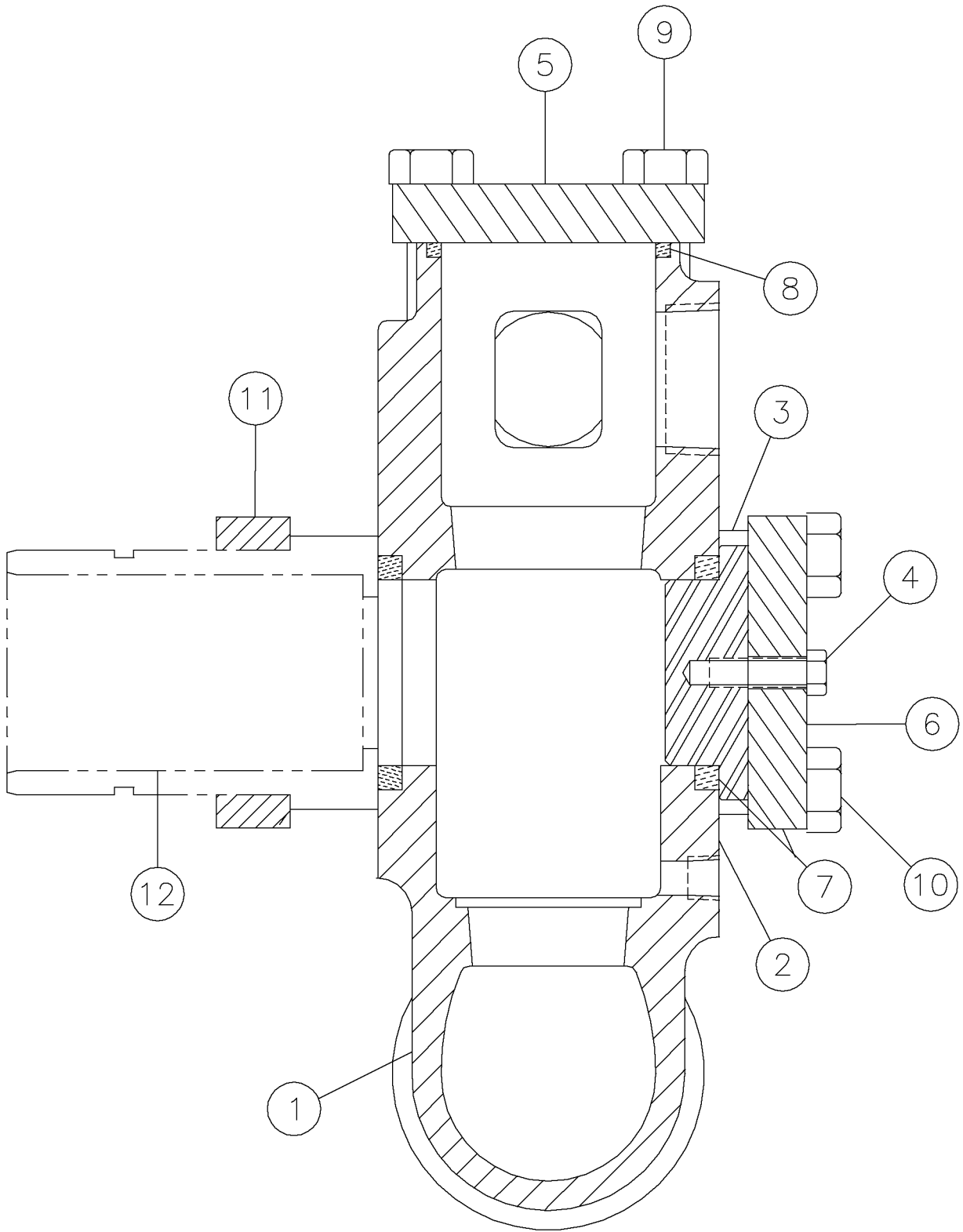
Components-Fluid End Fig 11-3z03
