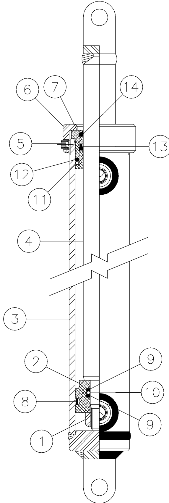
Components- Cylinder Fig 7-13z02
