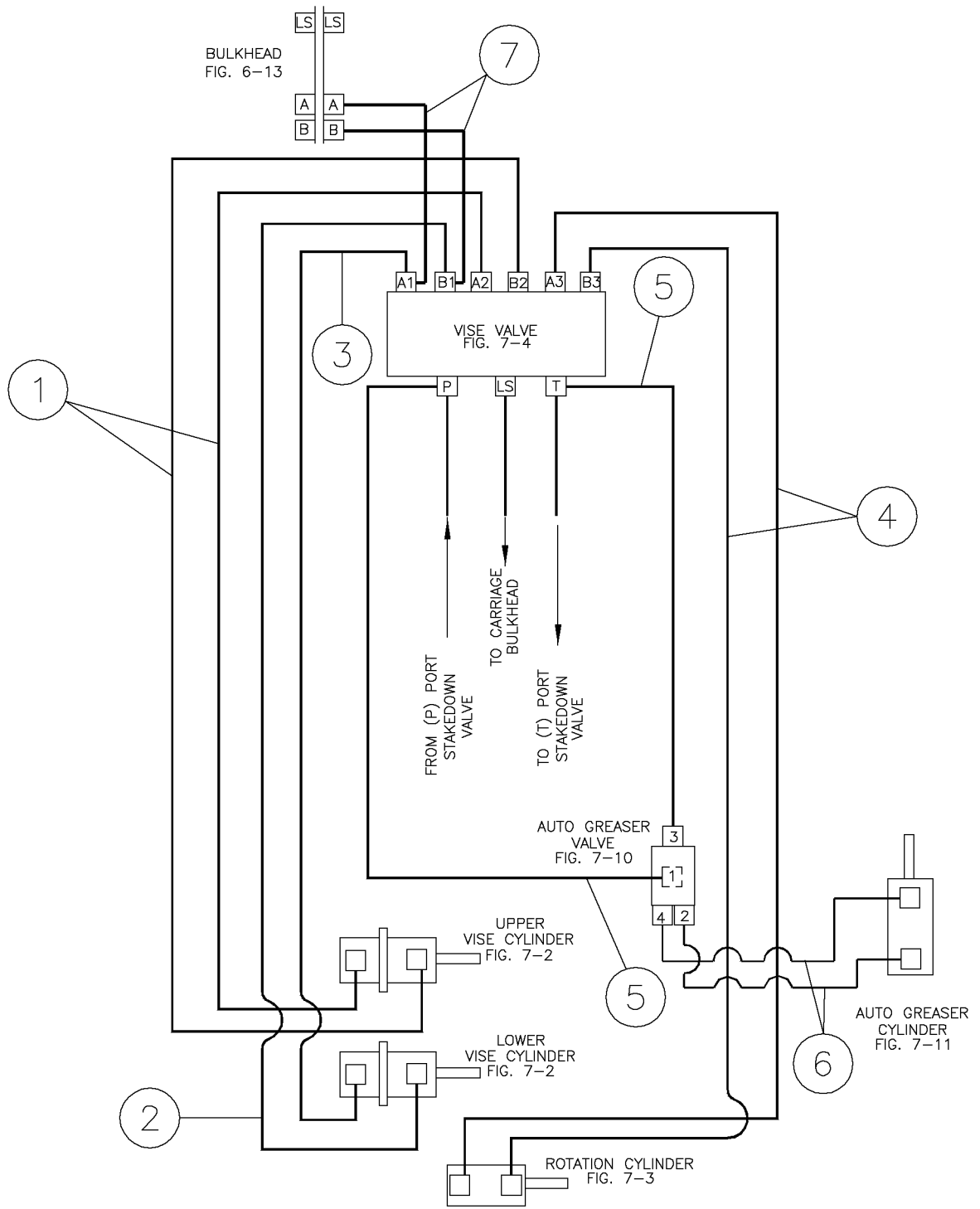
Vise Clamp Fig 12-6
