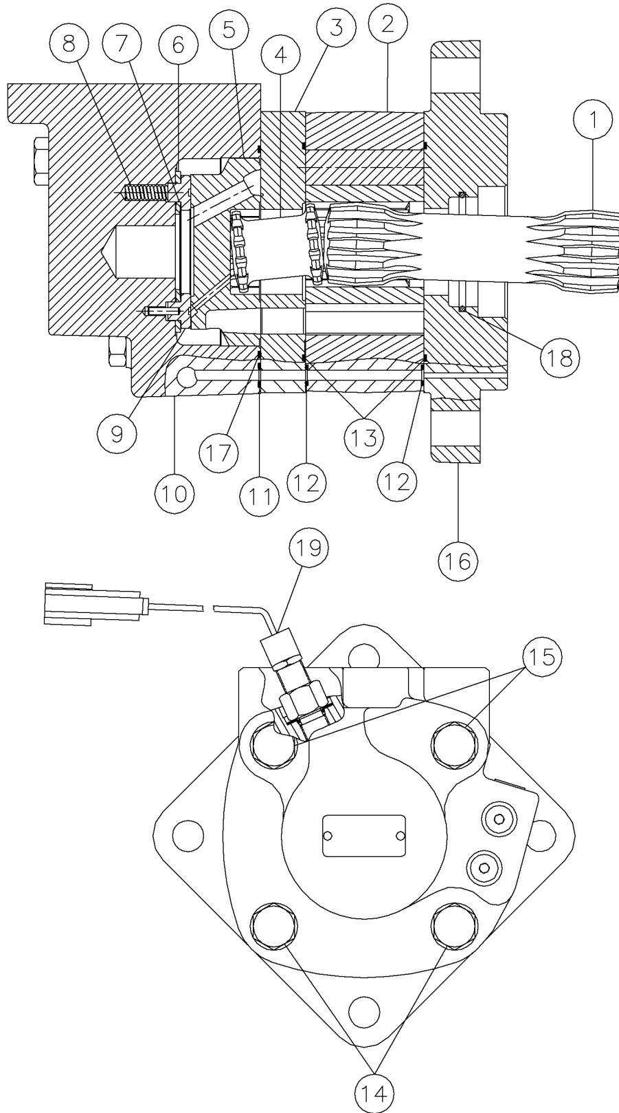
Components-Motor 70 GPM APLEX Fig 11-6z01
