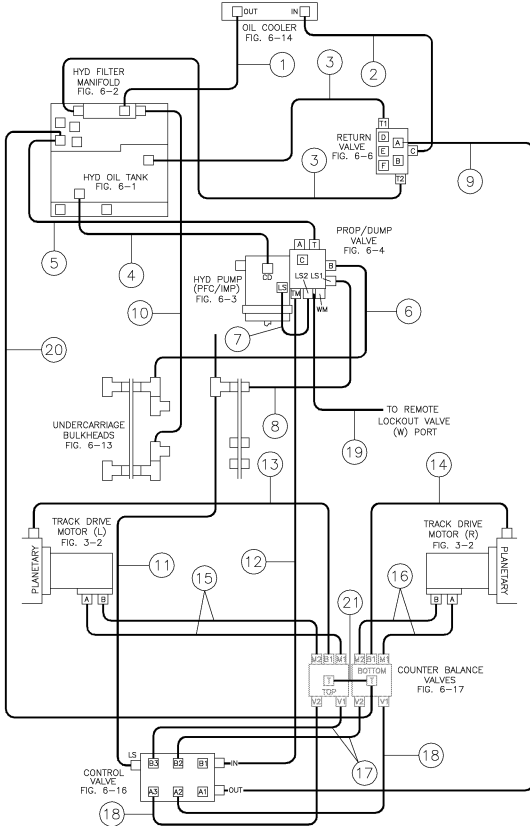
Ground Drive System Fig 12-4
