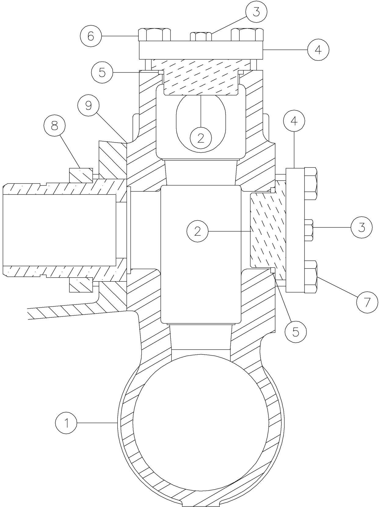
Components-Fluid End Fig 11-5z03
