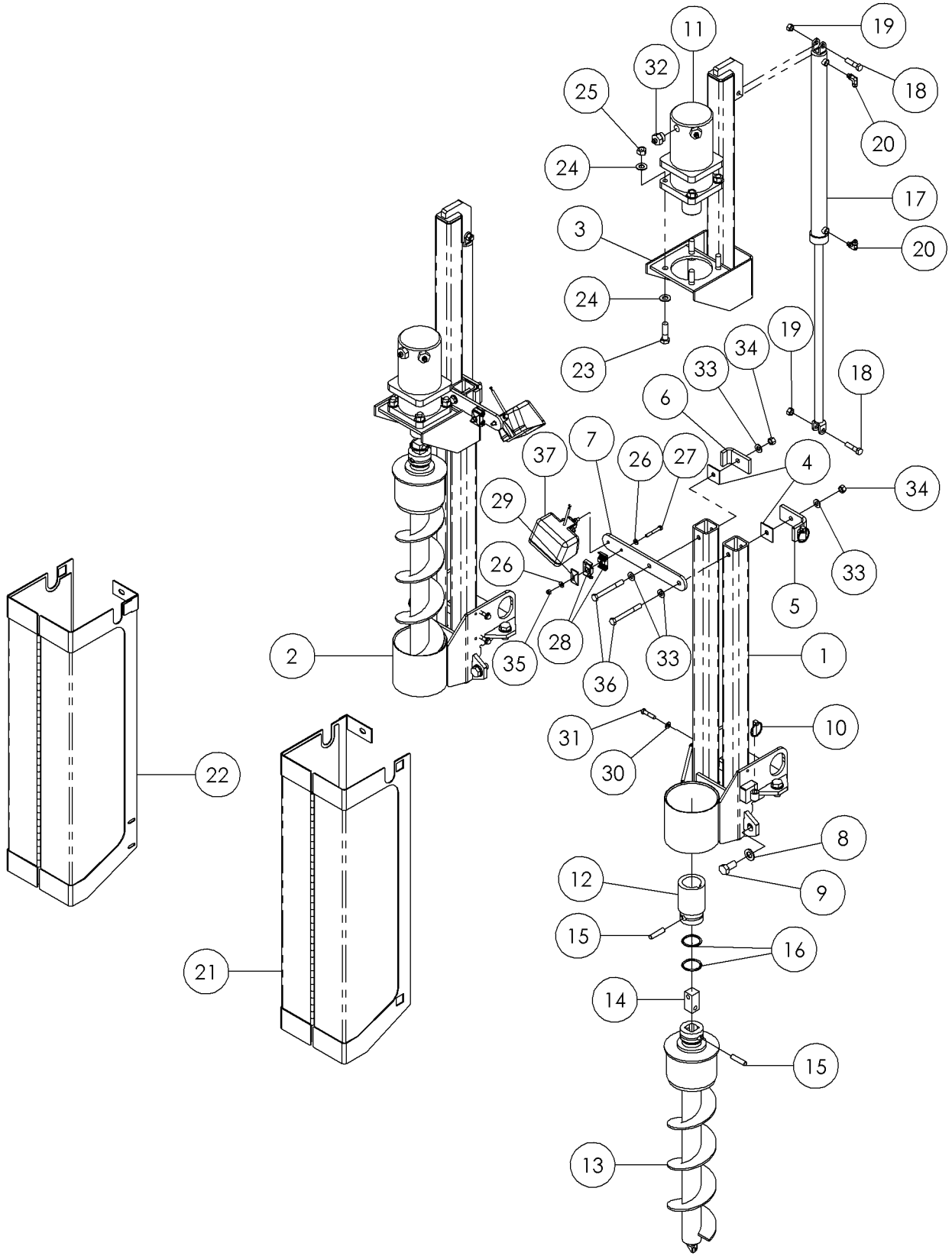
Stakedown (S/N 552-565) Fig 7-13
